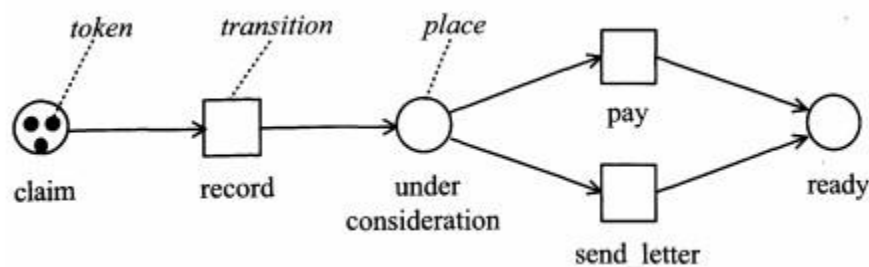
Gambar 3-1: Contoh petri net [4]
