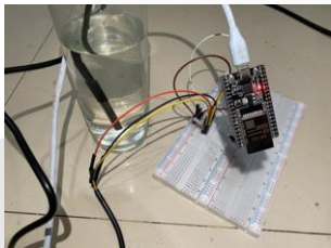
GAMBAR 3 Sensor Suhu DS18B20
