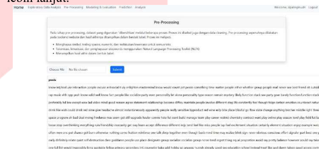
GAMBAR 11 Tahap Pre-Processing
