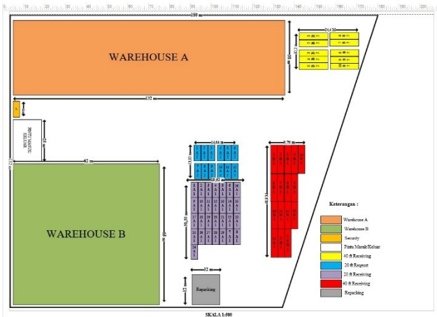
GAMBAR 3 LAYOUT ALTERNATIF 2 CLASS BASED MANUAL
