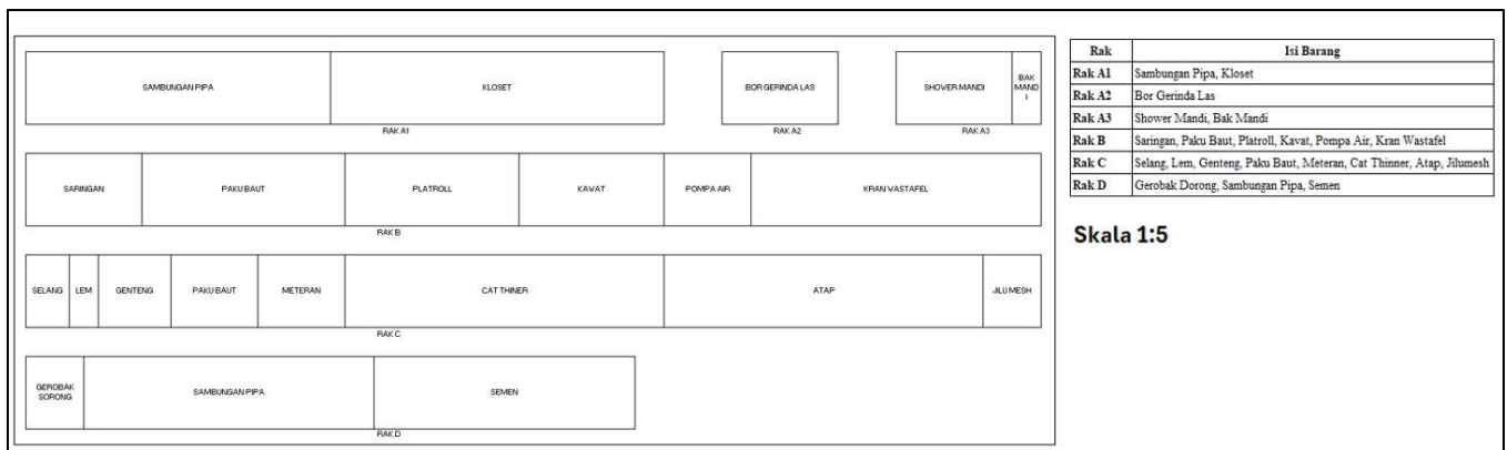
GAMBAR 5 LAYOUT RAK USULAN PT NBM
