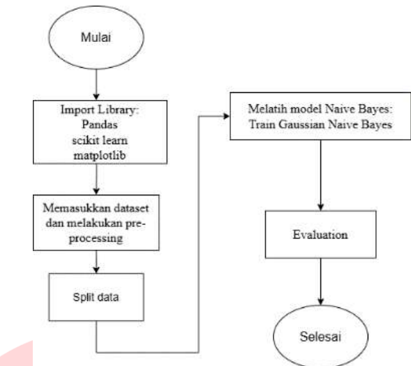
GAMBAR 3. DIAGRAM ALIR NAÏVE BAYES
