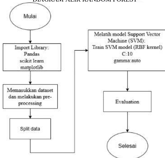
GAMBAR 2. DIAGRAM ALIR SUPPORT VECTOR MACHINE (SVM)
