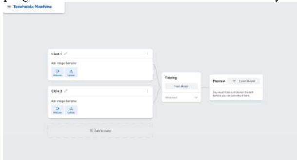
GAMBAR 8 (Teachable Machine)
