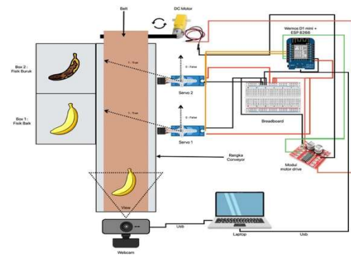
GAMBAR 11 (Rangkaian detail sistem)
