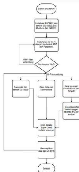
GAMBAR 2 Flowchart alur sistem IoT
