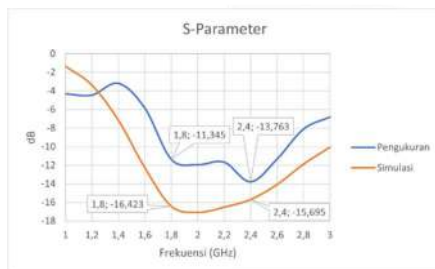
GAMBAR 12 Return loss
