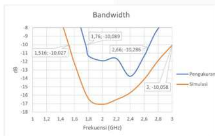
GAMBAR 13 Bandwidth
