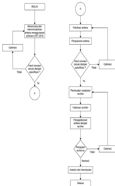
GAMBAR 4 (Flowchart implementasi sistem)
