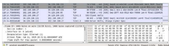
GAMBAR 9 Tampilan Wireshark
