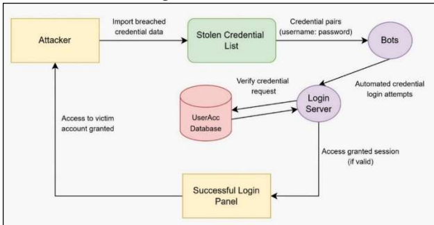
GAMBAR 3 Data flow diagram brute-force login
