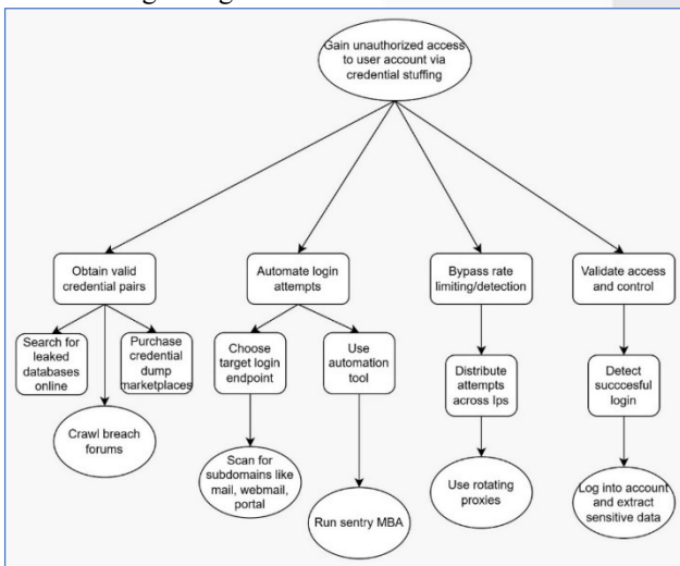
GAMBAR 4 Attack tree brute-force login
