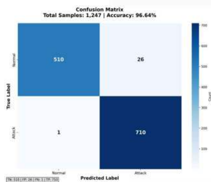
GAMBAR 4 Confusion Matrix
