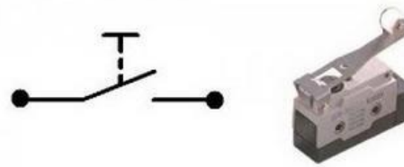
Gambar 2.5 Limit Switch
