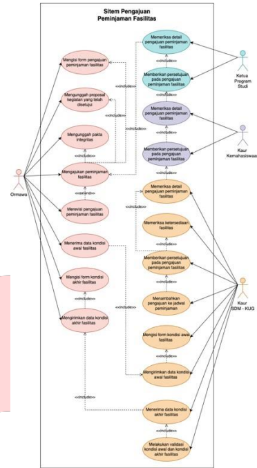
Gambar IV. 2 Use Case Diagram
