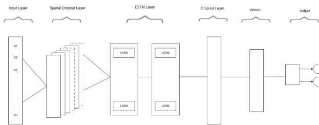
GAMBAR.4 LSTM Architecture
