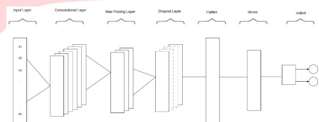
GAMBAR.3 CNN Architecture
