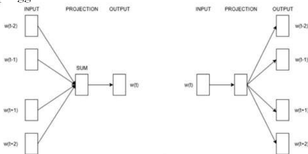
GAMBAR.2 Feature Expansion Word2vec
