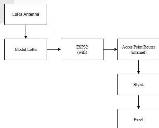
GAMBAR 2 (Blok Diagram Gateway)
