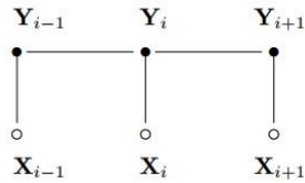
Gambar 1 Linear Chain Conditional Random Fields
