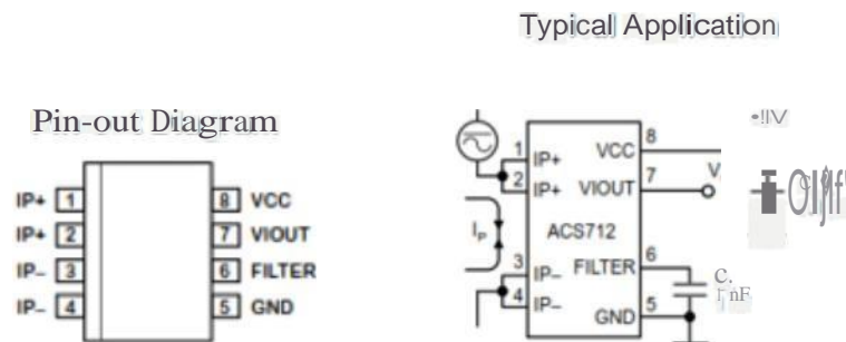
Gambar 5. Sensor Arus
