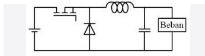
Gambar 2. Rangkaian Buck Converter.
