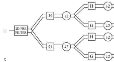
Gambar 2.2 Dekomposisi Multiwavelet Transformation
