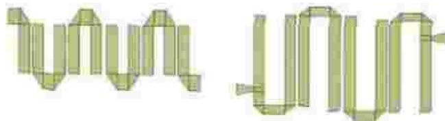
Gambar 6 Microstrip (a) Coupled Line Input (b) Tapped Line Input [7]
