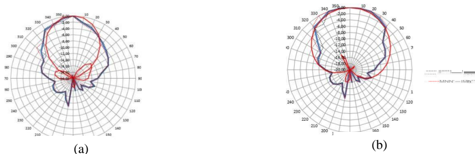
Gambar 9. Hasil Pengukuran Polaradiasi (a) Arah Azimuth, (b) Arah Elevasi.
