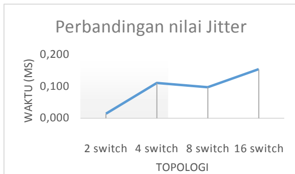
Gambar 3.1.2 Nilai Jitter
