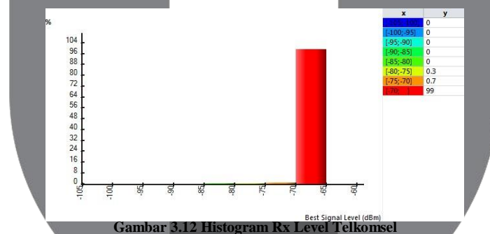
Gambar 3.12 Histogram Rx Level Telkomsel
