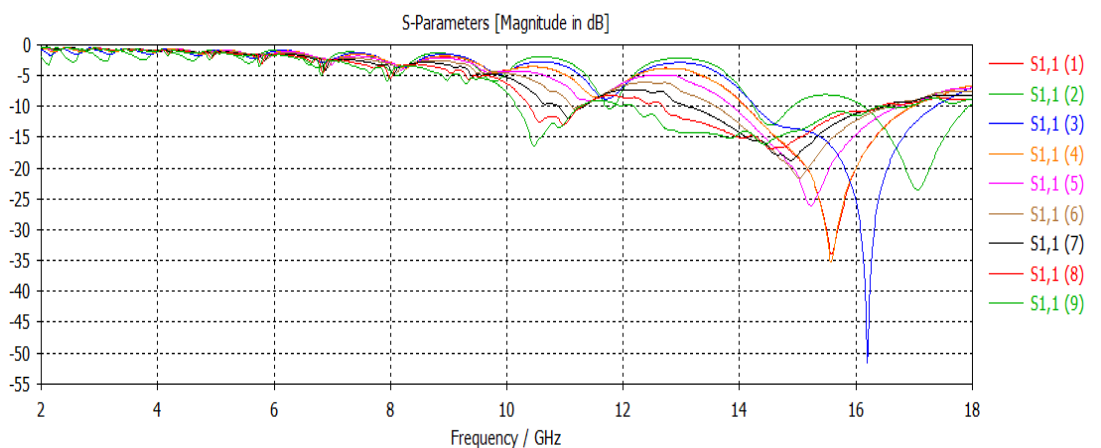
Gambar 3.2 Hasil Return Loss
