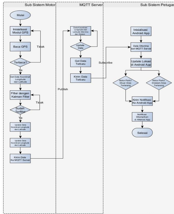
Gambar 3. Flowchart Sistem
