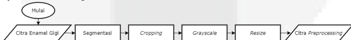
Gambar 4. Diagram alir preprocessing
