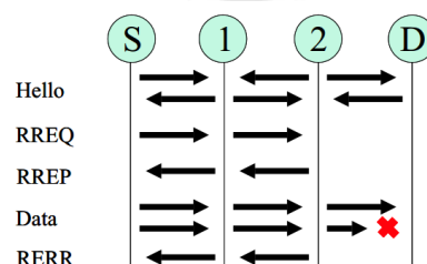
Gambar 1. Proses Pencarian Rute AODV
