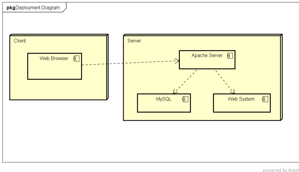
Gambar 4.1 Deployment Diagram
