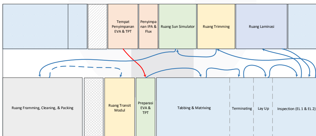
Gambar 3 Spaghetti Diagram
