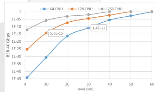
Gambar 6 BER 40 Gbps Upstream
