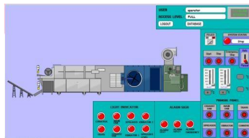
Gambar 13 Workstation Window
