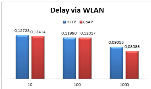
Gambar 6. Grafik Delay via WLAN
