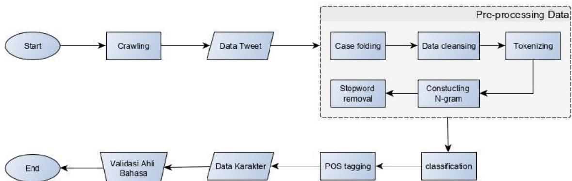
Gambar 2 Blok Diagram POS tagging
