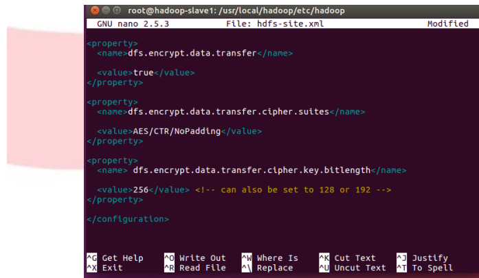
Gambar 4.4 Implementasi HDFS Data Transfer Protocol Encryption
