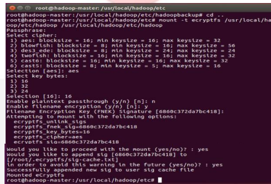
Gambar 4.2 Implementasi Filesystem Encryption
