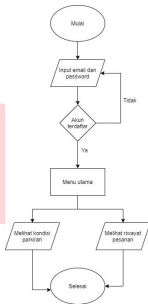
Gambar 3. 2 Flowchart Admin
