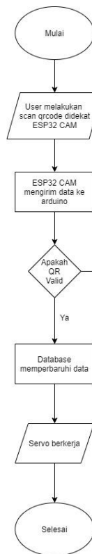
Gambar 3. 3 Flowchart Alat
