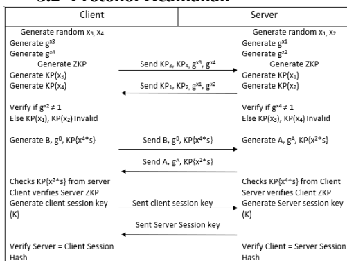
Gambar 2 Diagram J-PAKE
