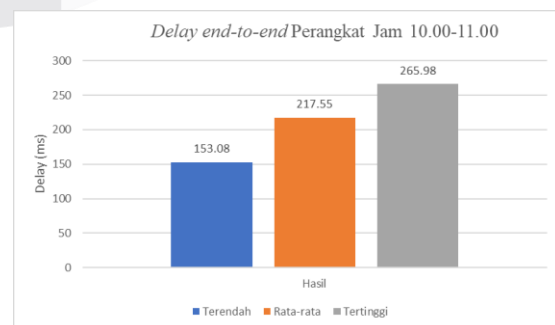
Gambar 10. Hasil Delay Jam 10.00-11.00
