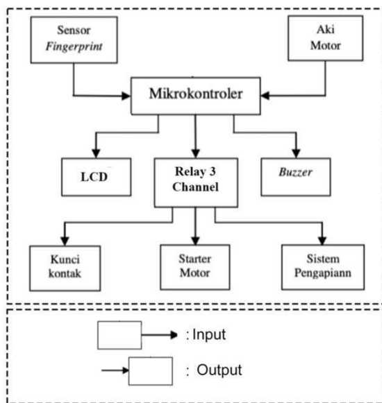
GAMBAR 3.3 Blok Diagram
