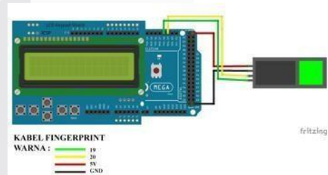
GAMBAR 3.5 Skematik Fingerprint
