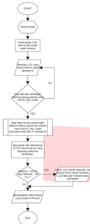
Gambar III- 4 Diagram Alir Dashboard Kendaraan ( Receiver )
