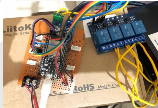
GAMBAR 2 (Sistem Kendali Arus berbasis Internet of Things )
