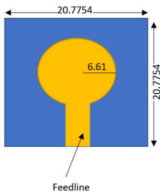
GAMBAR 3. 3 (Gambar Antena Patch Circular Simulasi.)
