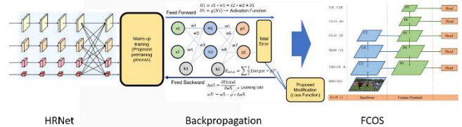
FIG 9 (The proposed training flow on the model.)
