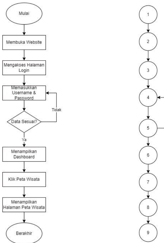
GAMBAR 18 (FLOWCHART & FLOW GRAPH PETA WISATA)
