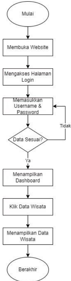
GAMBAR 17 (FLOWCHART & FLOW GRAPH DATA WISATA)
