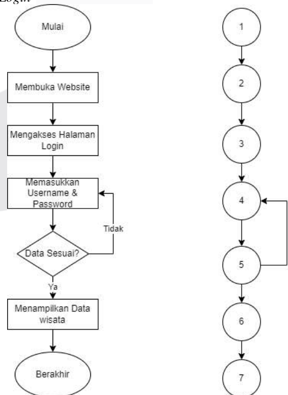
GAMBAR 16 (FLOWCHART & FLOW GRAPH LOGIN)
