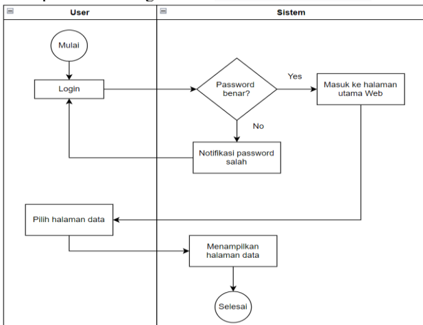
GAMBAR 5 (ACTIVITY DIAGRAM)
