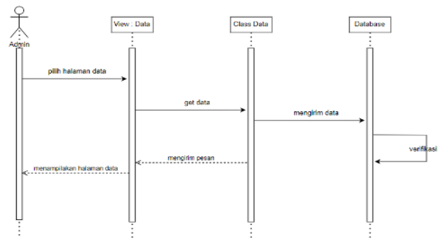
GAMBAR 6 (SEQUENCE DIAGRAM)
