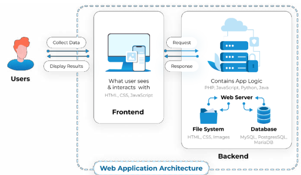
GAMBAR 2. 3 WEB APPLICATION ARCHITECTURE
