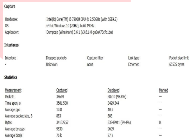
GAMBAR 7 HASIL PACKET CAPTURE EXISTING
