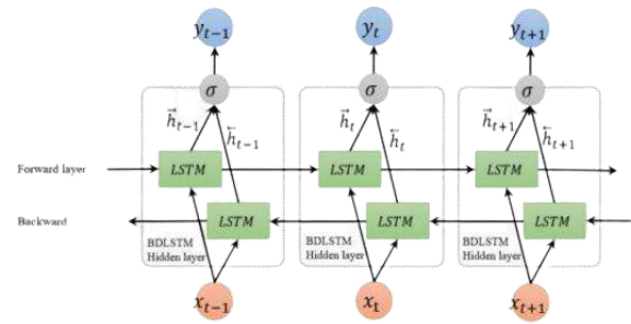
FIGURE 3 ARSITEKTUR BIDIRECTIONAL LSTM[11]
