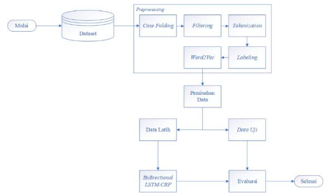
FIGURE 5 ARSITEKTUR SISTEM BIDIRECTIONAL LSTM-CRF
