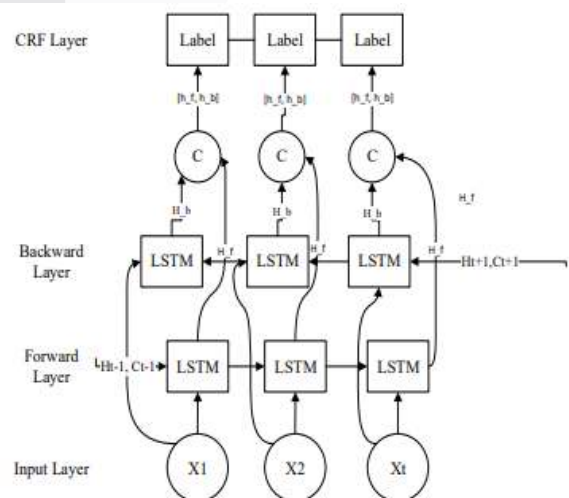
FIGURE 4 ARSITEKTUR BIDIRECTIONAL LSTM-CRF[13]
