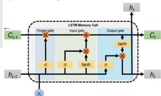
FIGURE 2 LSTM MEMORY CELL[7]
