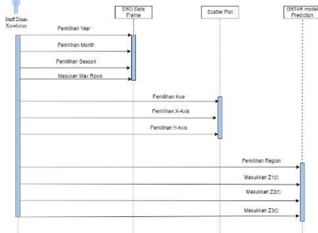
Gambar 2. Sequence Diagram
