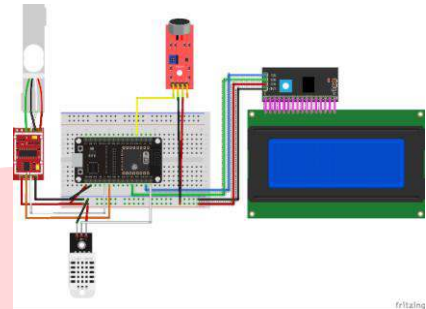
GAMBAR 14 Wiring Diagram
