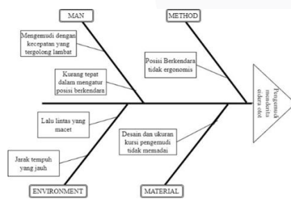
GAMBAR 3 (Fishbone Diagram)
